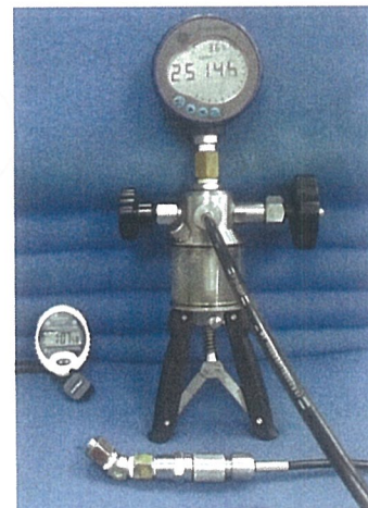
Hydrostatic Test
