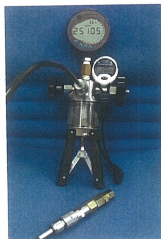
Hydrostatic Test
